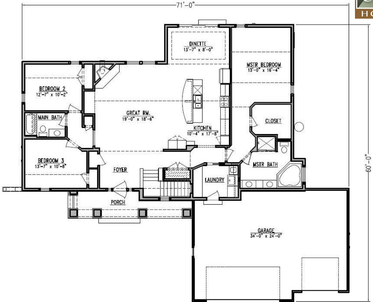
MODEL PLAN AS BUILT WITH PRE-DESIGNED OPTIONS – 1,938 S.F.
